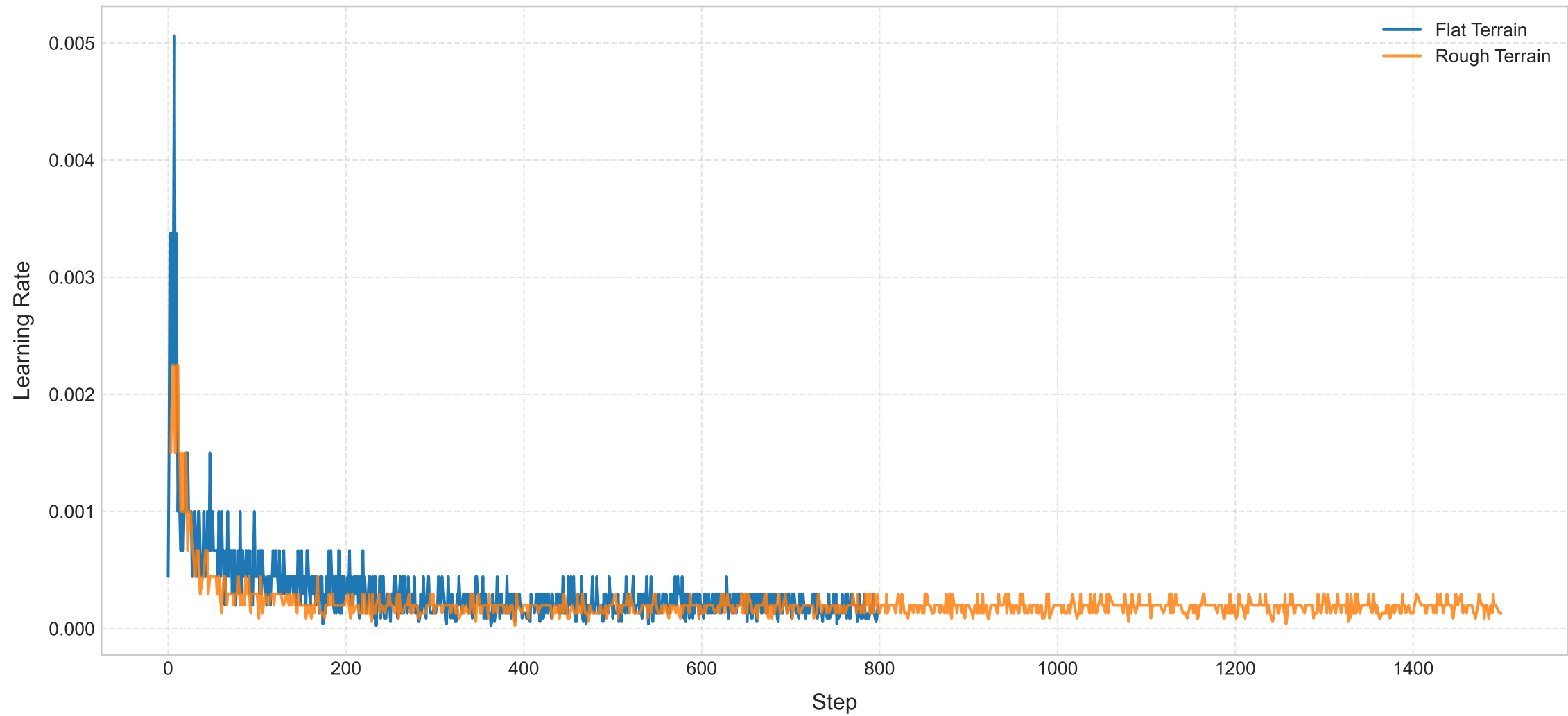
Adaptive Learning Rate
